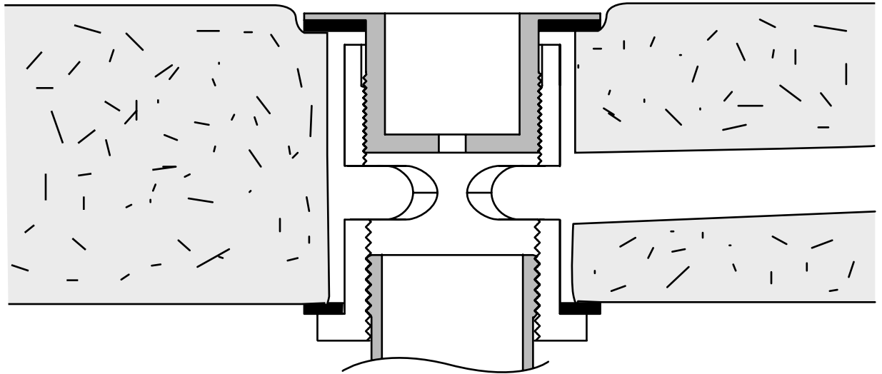
Installed section view showing overflow
